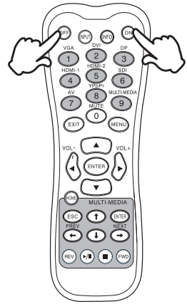
[Remote Control]
